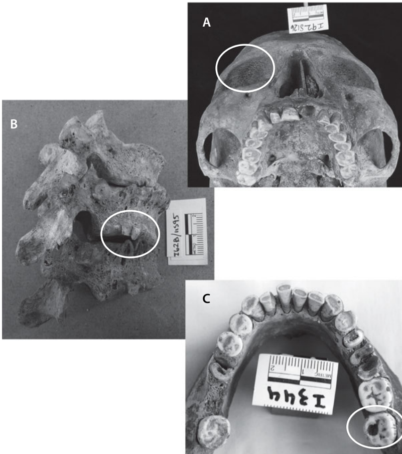
7.3. Paleopathological markers. A. cribra orbitalia; B. osteoarthritis; C. dental caries. All examples stem from the ancient city of Amarna in Egypt. Images courtesy of Jerry Rose.
