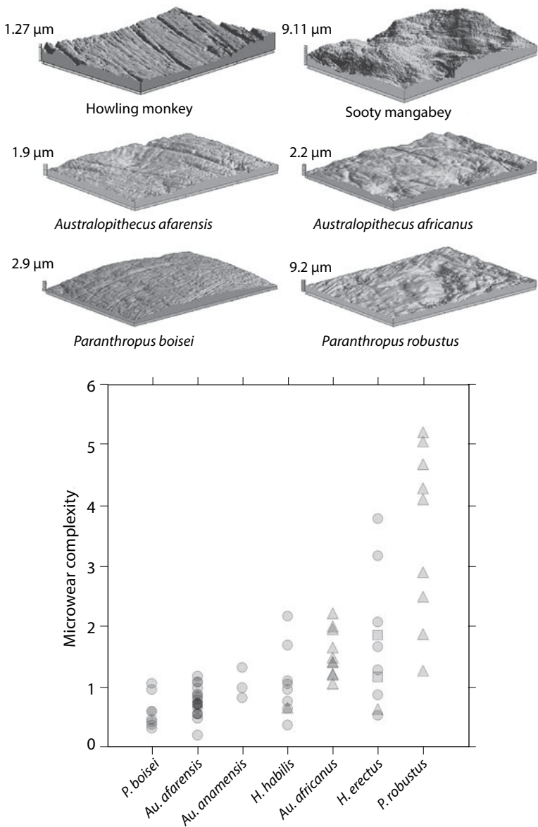
5.2. Dental microwear photosimulations of tooth areas 0.10 \times 0.14 mm ( top ) and microwear texture complexity data for Plio-Pleistocene hominins ( bottom ). Eastern African hominin specimens are represented by gray circles, South African ones by triangles, and Asian ones by squares.
