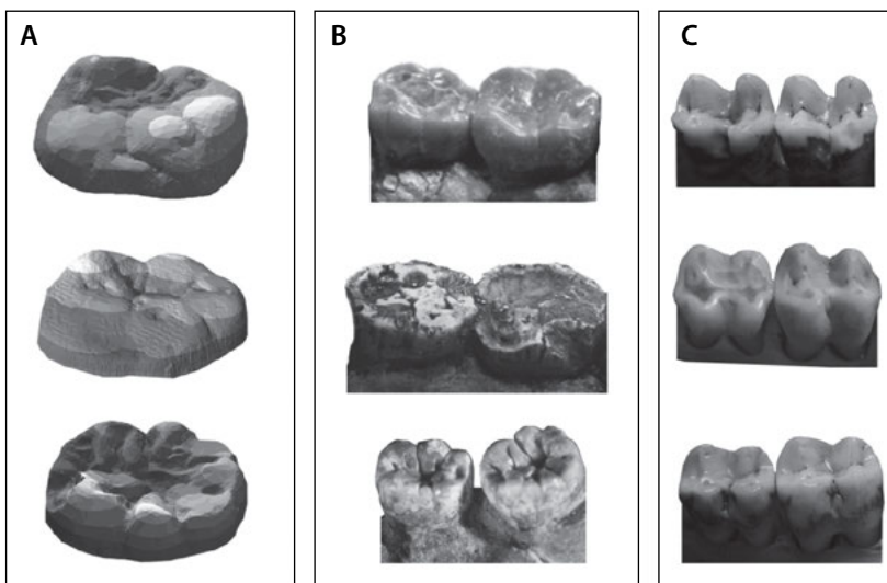
1.4. Dental topography. A. GIS models of molar teeth of fossil hominins Australopithecus afarensis , Paranthropus boisei , and Homo erectus ; B. photographs of molars of those same species; C. photographs of molar teeth of a leaf monkey ( above ), a frugivorous macaque ( middle ), and a hard-object feeding mangabey ( below ).
