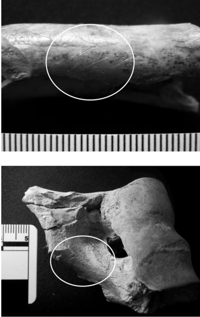
6.2. Upper-arm-bone fragments of antelopes from the Zinjanthropus site at Olduvai Gorge. Note the cut marks indicated by the circles. Images courtesy of Henry Bunn.
