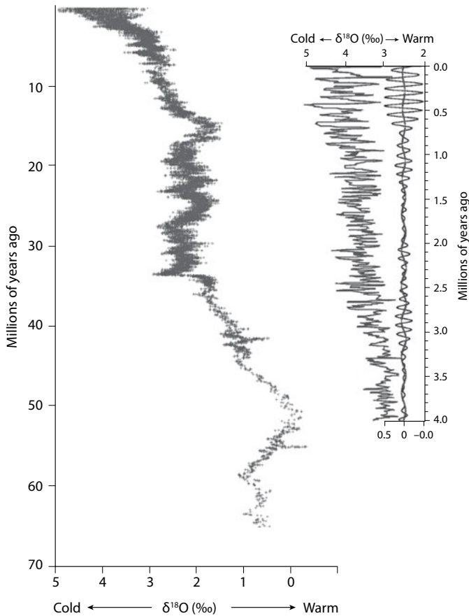
4.3. Northern hemisphere paleoclimate data based on oxygen isotopes. The larger graph represents temperature trends over the Cenozoic era and the smaller one represents the past four million years. The rightmost graphic measures variance associated with eccentricity cycles. Modified with permission of James Zachos (see James Zachos, et al., “Trends, Rhythms, and Aberrations in Global Climate 65 Ma to Present,” Science 292, no. 5517 (2001): 686–93, and James Zachos, Gerald Dickens, and Richard Zeebe, “An Early Cenozoic Perspective on Greenhouse Warming and Carbon-Cycle Dynamics,” Nature 451, no. 7176 (2008): 279–83, for details).
