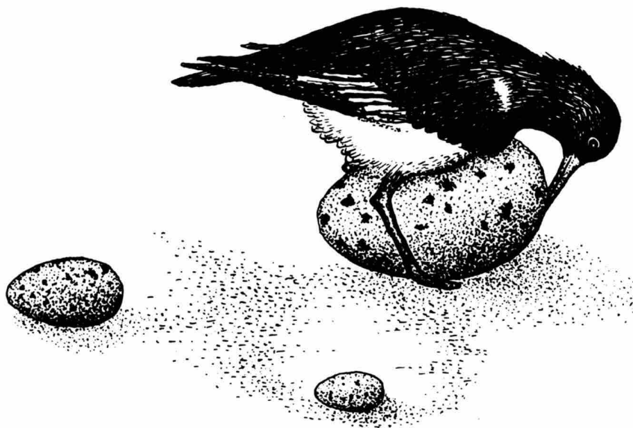
Figure 48. Oystercatcher Responding to a “Supernormal Stimulus”
