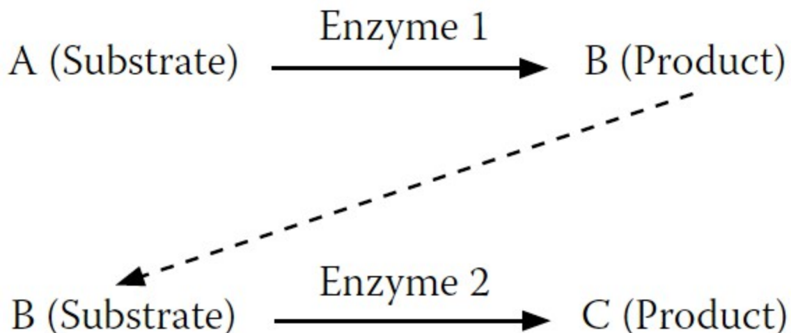
FIGURE 7-4. A simple enzyme reaction
