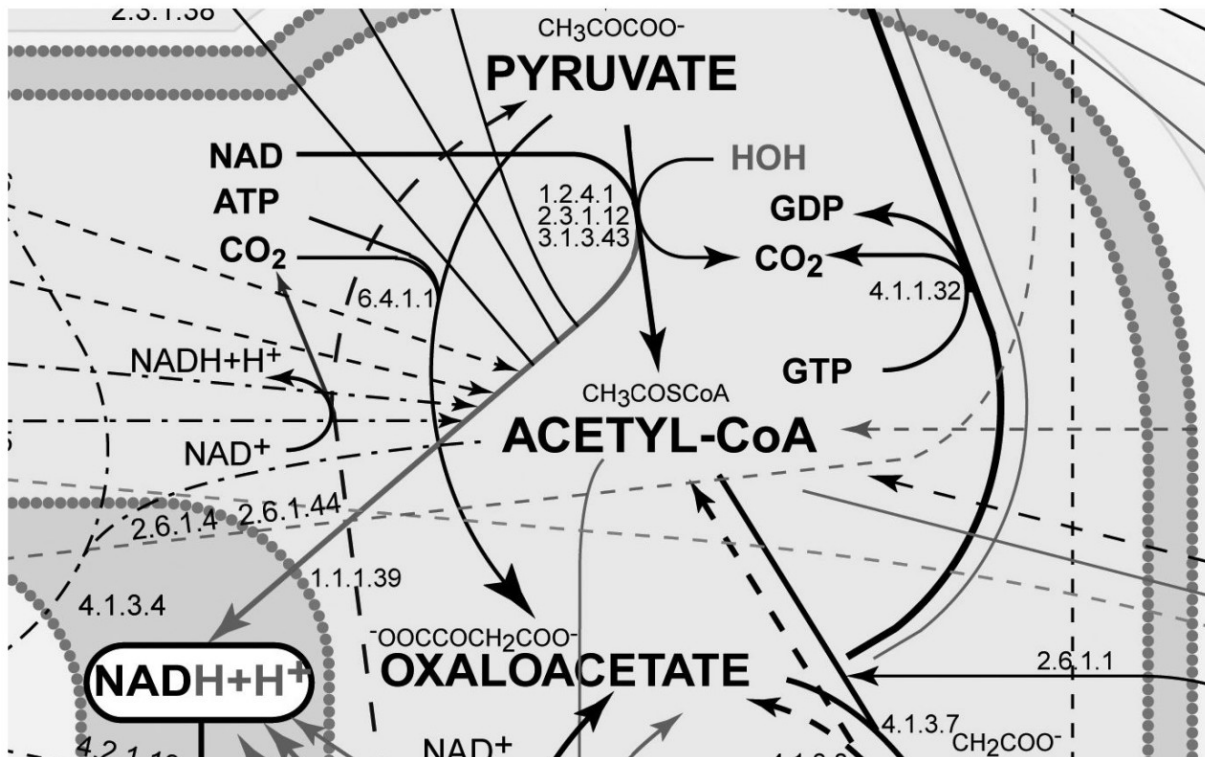
FIGURE 7-3. Expanded inset of Figure 7-2
