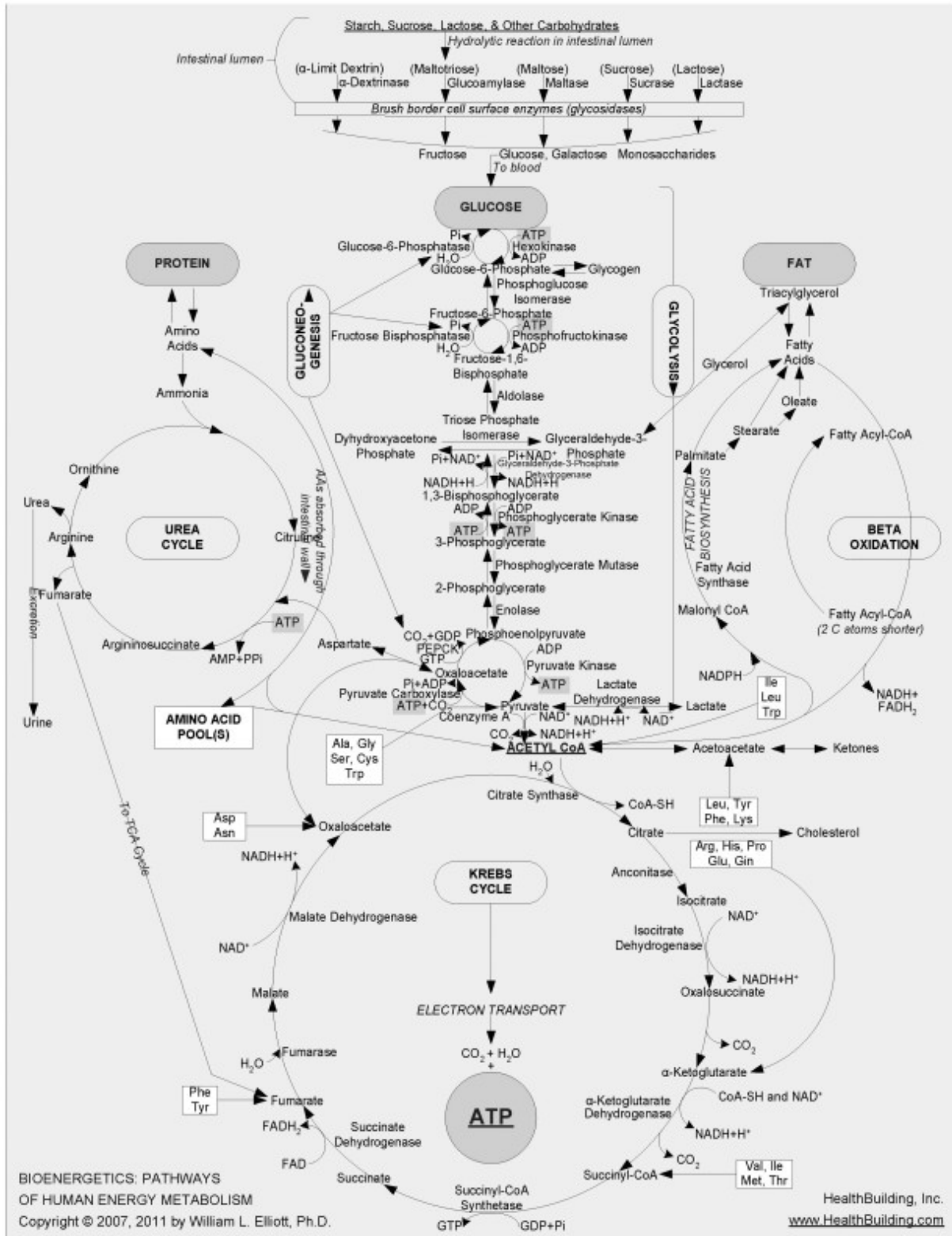
FIGURE 7-1. Chart mapping glucose metabolism and other metabolic pathways 20
