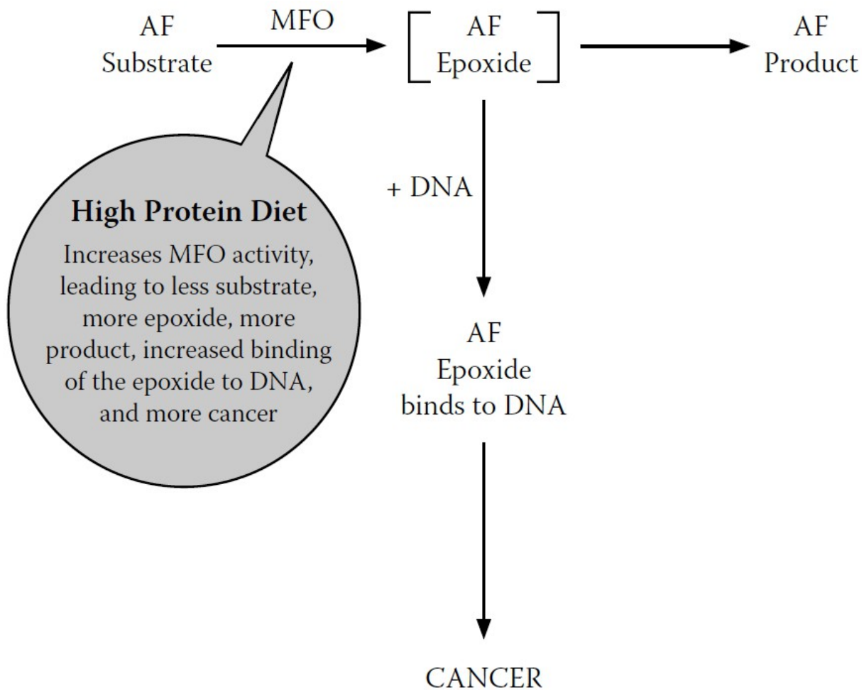
FIGURE 7-8. Final revised model for MFO conversion of AF
