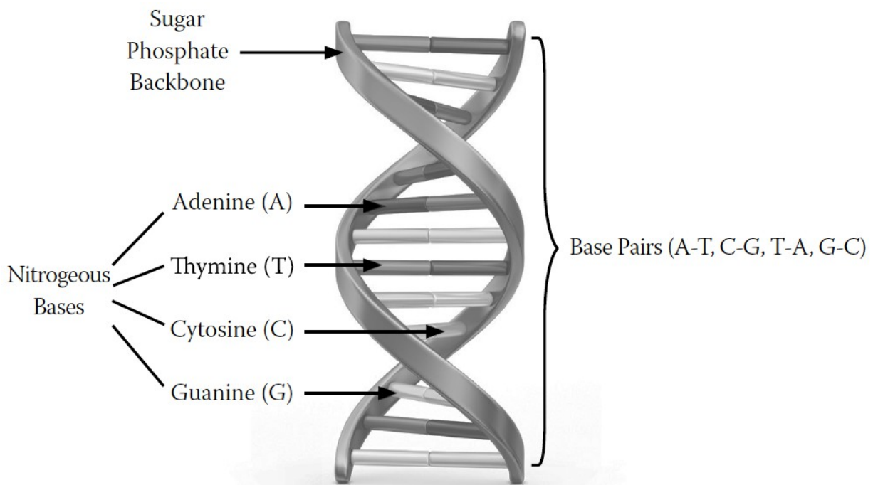
FIGURE 8-1. A DNA molecule
